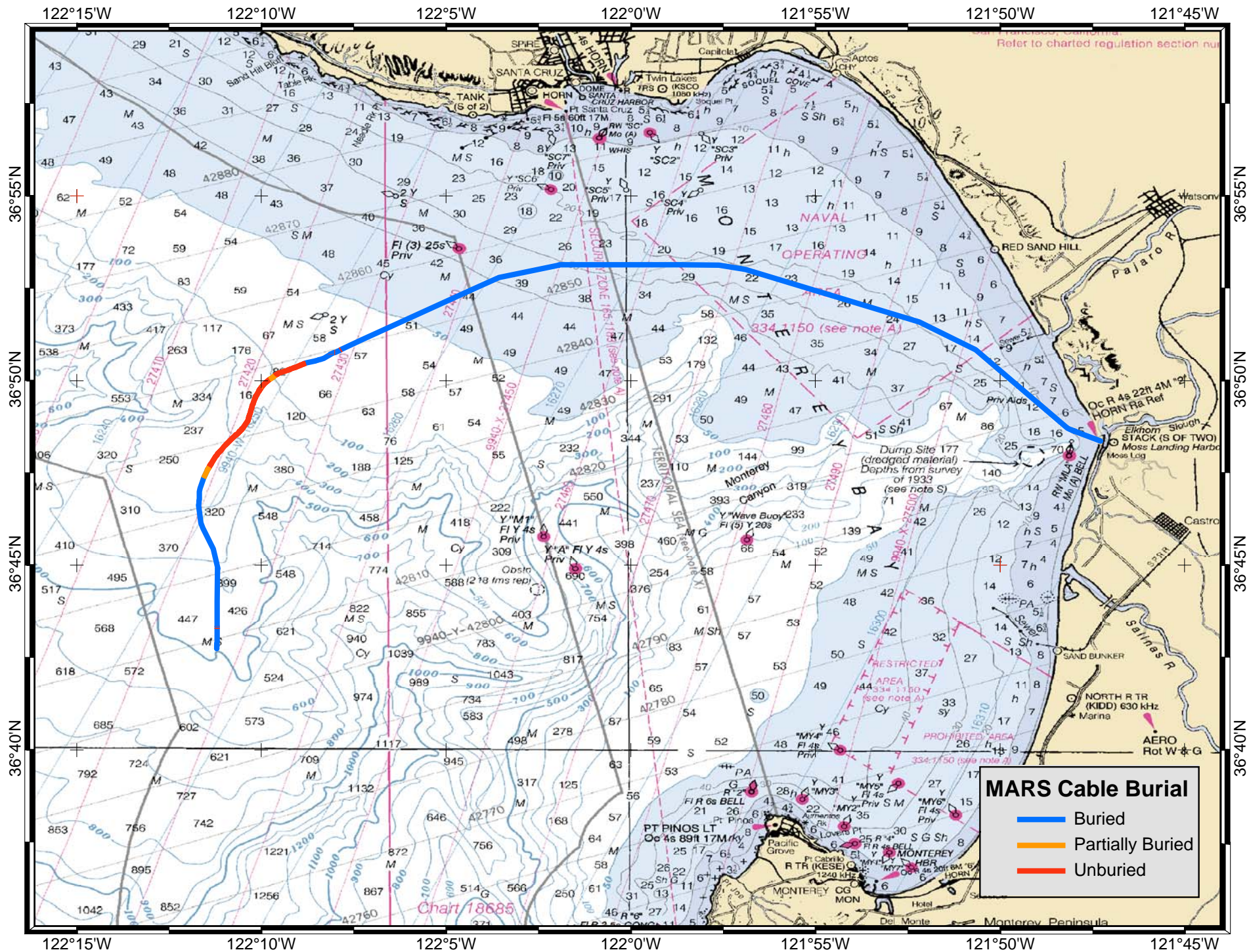
The MARS cable route is indicated by the colored line from Moss Landing, CA out into Monterey Bay. Blue portions are buried, orange portions are partially buried, and red portions are unburied sections of cable. (Image is not intended for navigational purposes.)
